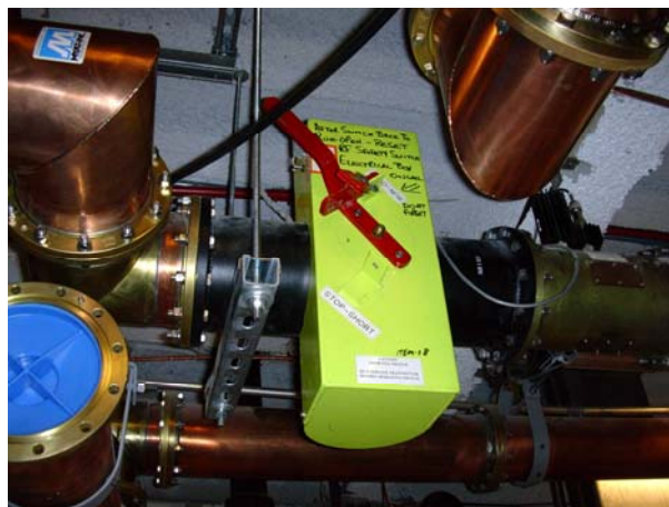
Figure 16. A manual patch is used to isolate the main combiner feed from either the main or backup antenna. The lockout/tagout switch preceding the patch assures that there is no RF energy present, before the patch can be pulled and moved.
